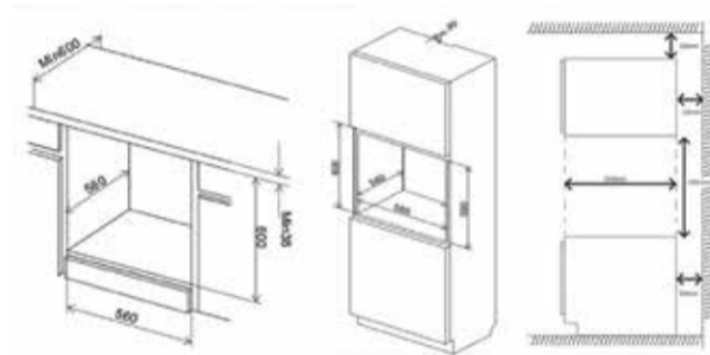
BO710M1 / BO810D1 Multifunctional Oven
