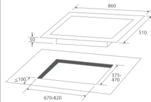
KGH93SG 90cm Gas Hob W670-820 x D375-470^
