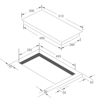
KGH310SG 30cm Gas Hob W285 x D495^
