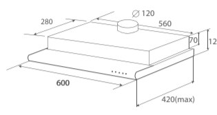
KSL66 60cm Telescopic Hood W600 x H120 x D420
