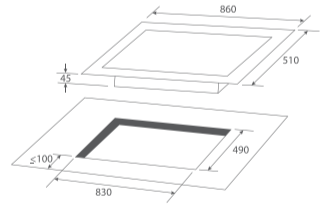
KGH93X 90cm Gas Hob W830 x D360-490
