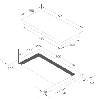
ID-30 30cm Induction Hob W270 x D500^
