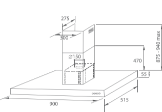
KCW598X 90cm Chimney Hood W900 x H940 x D515
