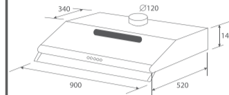
KSL94 90cm Slimline Hood W900 x H140 x D520
