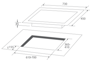
KGH72SG 72cm Gas Hob W610-700 x D360-410^
