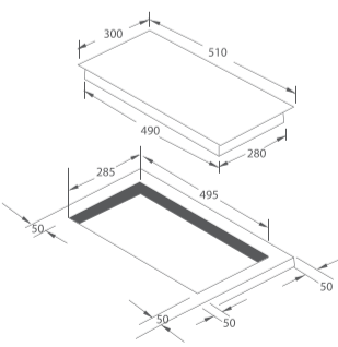
KGH320SG 30cm Gas Hob W285 x D495^
