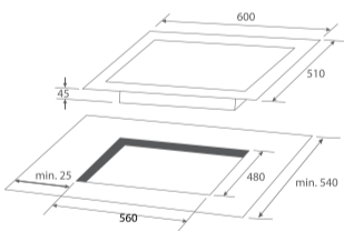
KGH630X 72cm Gas Hob W560 x D480^
