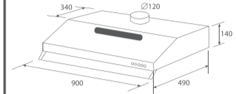
KSL95E 90cm Slimline Hood W900 x H140 x D490
